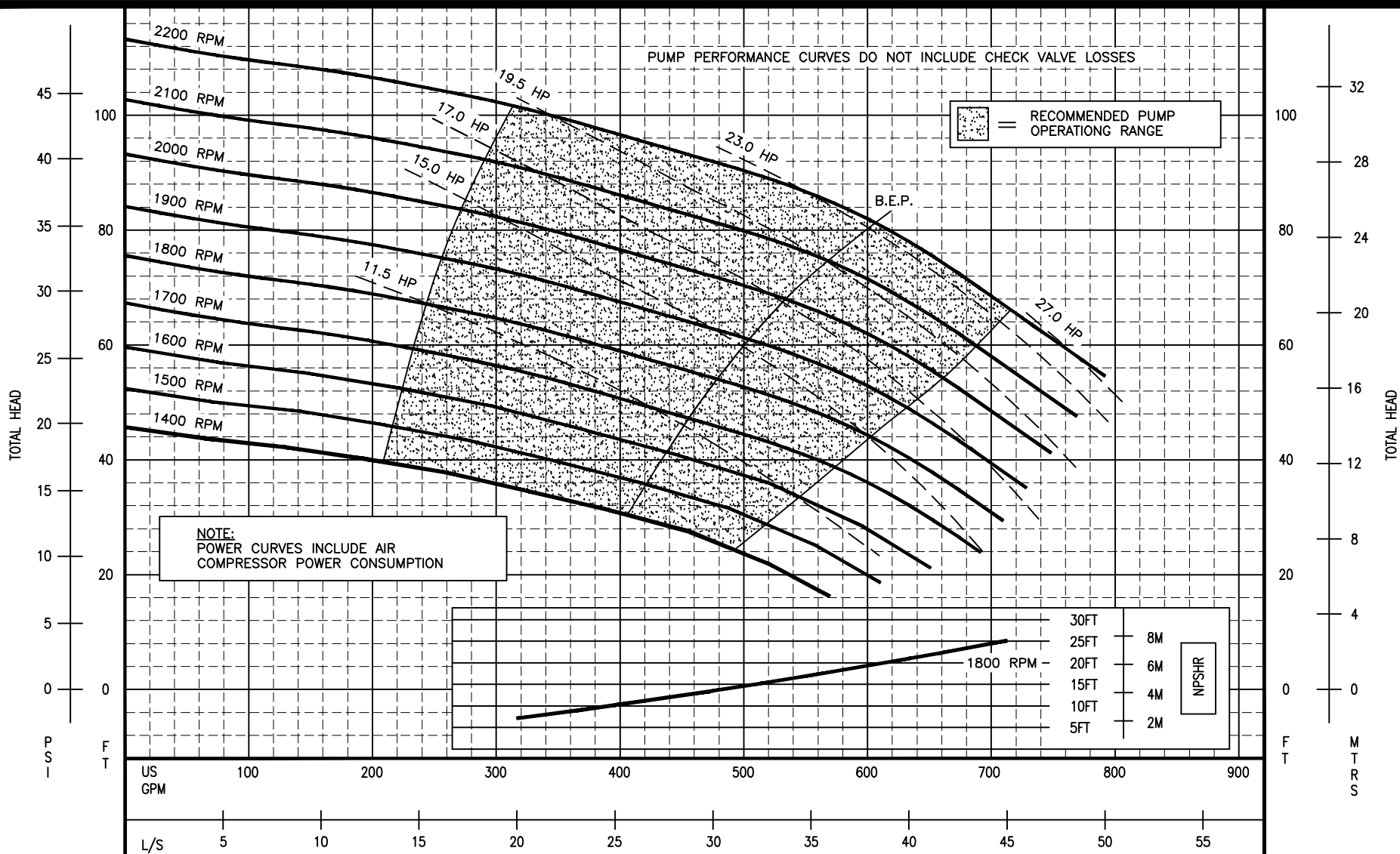
FLOW - CLEAR WATER PERFORMANCE
